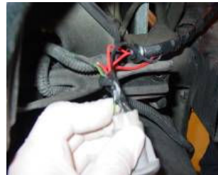
Step 17: Splice the red wires to the corner light, one red to power and other to ground.
